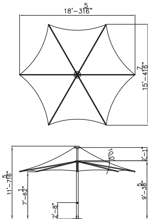
CODE: S56H SUNSET 18 FT. HEXAGONAL UMBRELLA
