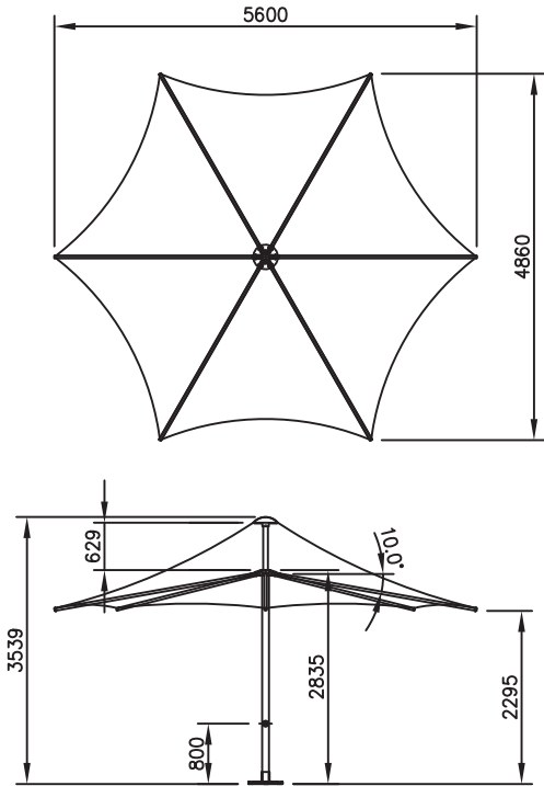
CODE: S56H SUNSET 5.0 M HEXAGONAL UMBRELLA
